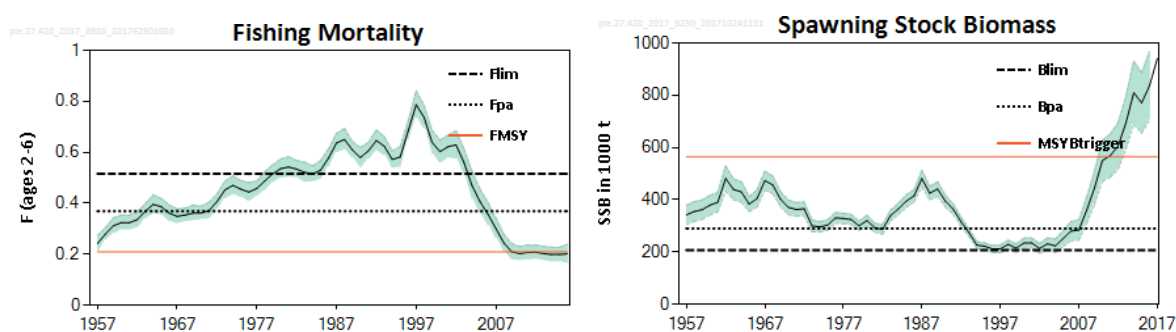
Fig. 1. Plaice in North Sea and Skagerrak. Summary of the stock assessment. Shaded areas (F, SSB) indicate \pm 2 standard errors (approximately 95% confidence intervals) (ICES Advice 2017).
