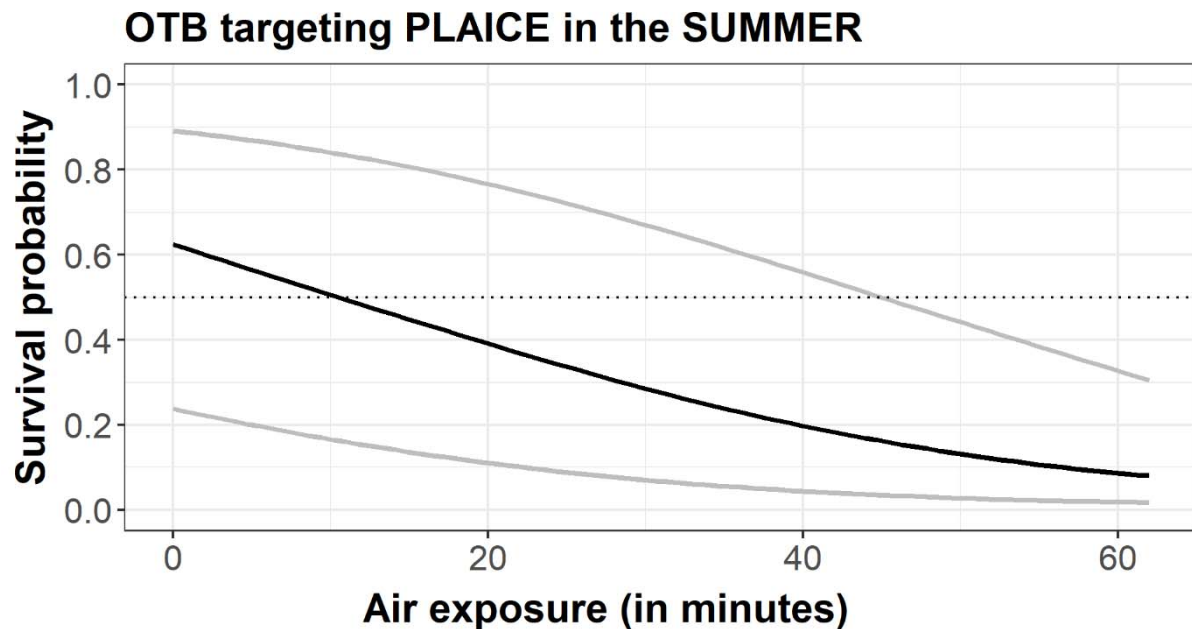
Fig. 5. Discard survival as a function of air exposure (black) with 95% confidence intervals estimated by parametric bootstrap accounting for variability from the captivity experiment (grey) for undersized plaice caught by the OTB targeting plaice in the summer.
