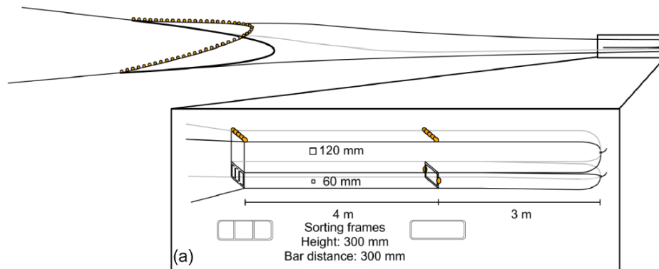
Fig. 3. A conceptual drawing of the horizontally divided codend used as one of the codends in the twin-rig of the trawler in the winter.
